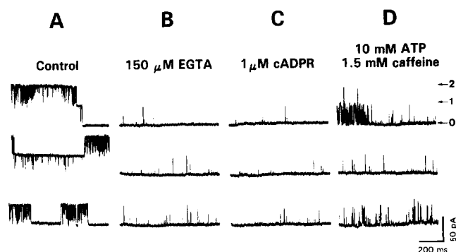
Fig. 2. Absence of cADPR effect on porcine cardiac RYR channels incorporated into lipid bilayers. Representative 858 ms traces are shown under control conditions (A, pCa 5; P_o = 22\% ) and following subsequent additions of 150 \mu\text{M} EGTA (B, pCa 8; P_o = 0.2\% ), 1 \mu\text{M} cADPR (C, P_o = 0.1\% ), and 1.5 mM caffeine and 10 mM ATP (D, P_o = 0.8\% ). Arrows at the upper right indicate current amplitudes for 0, 1, and 2 open channels. Records are from an experiment performed in the presence of symmetric 400 mM cesium methylsulfonate, 20 mM HEPES, pH 7.2, at a potential of +70 mV.
